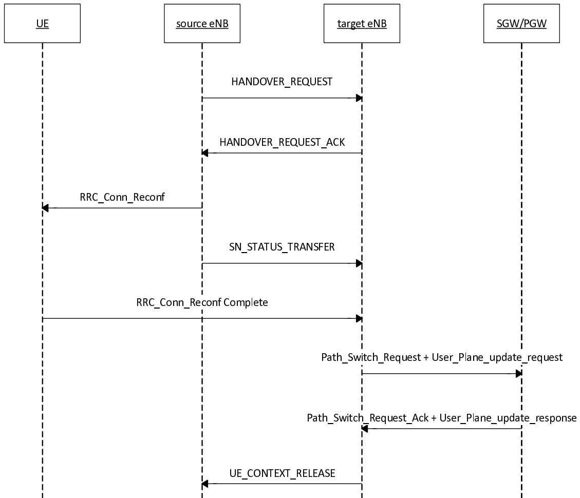
Figure 17.39: Sequence diagram of the X2-based handover
