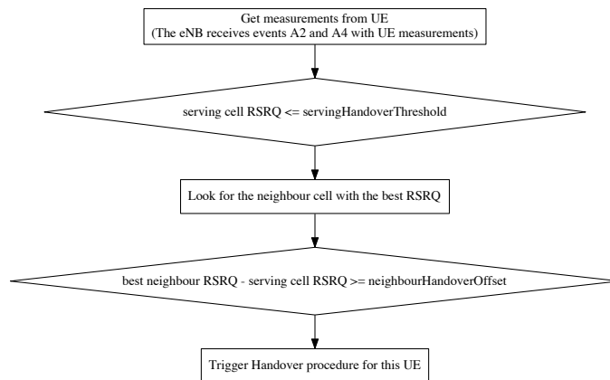
Figure 17.32: Algorithm to automatically trigger the Handover procedure
