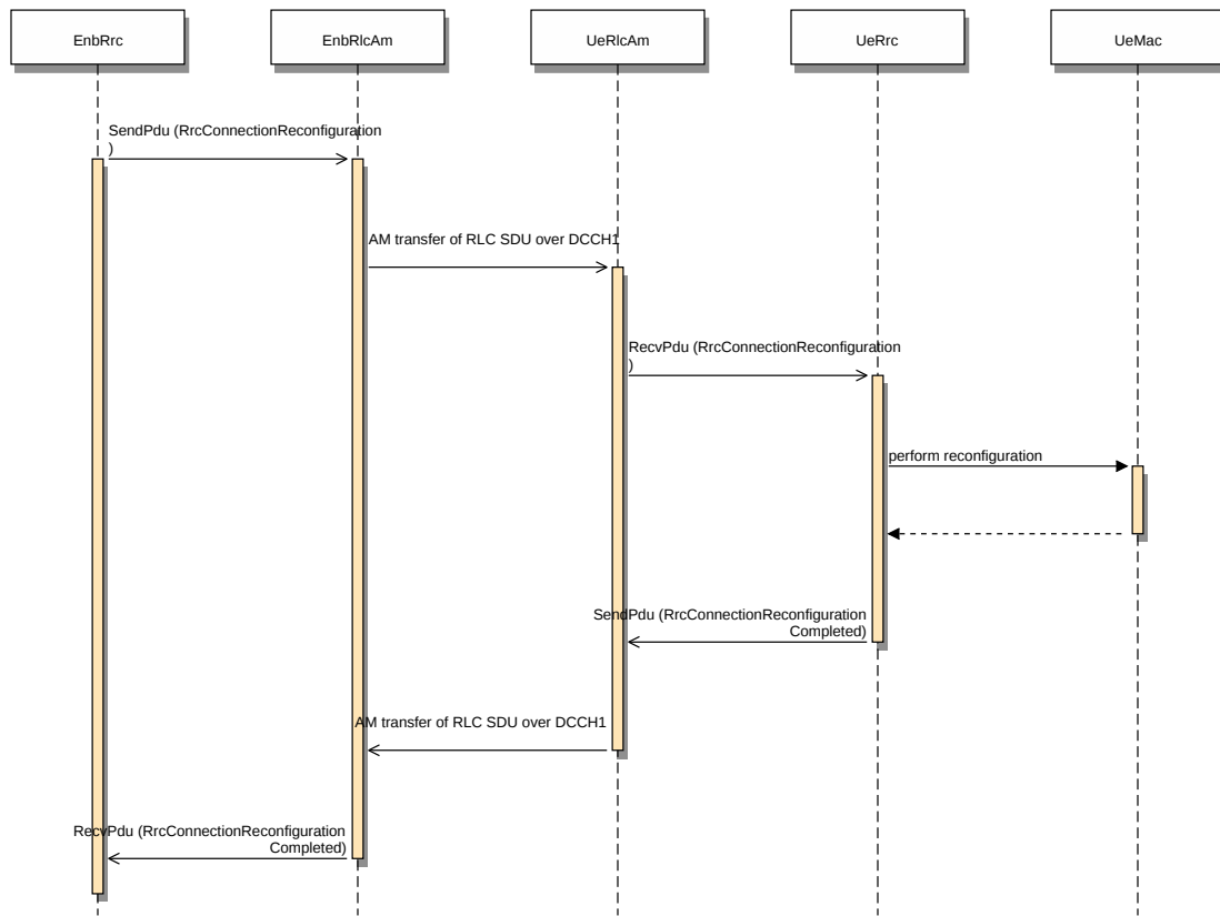
Figure 17.34: Sequence diagram of the RRC Connection Reconfiguration procedure
