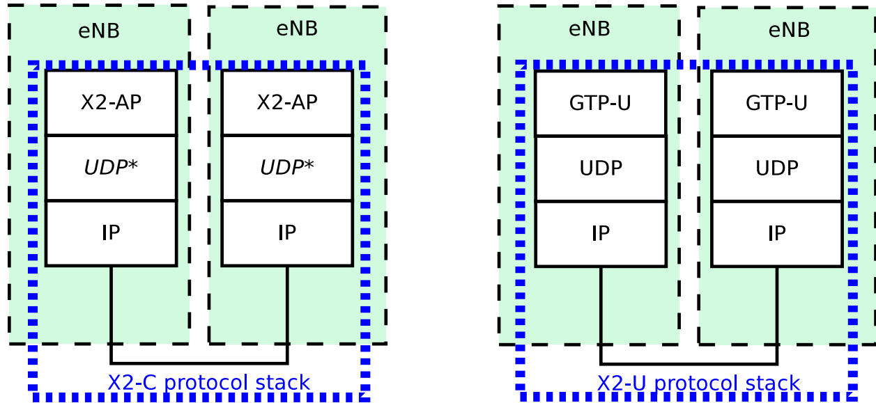
Figure 17.41: X2 interface protocol stacks
