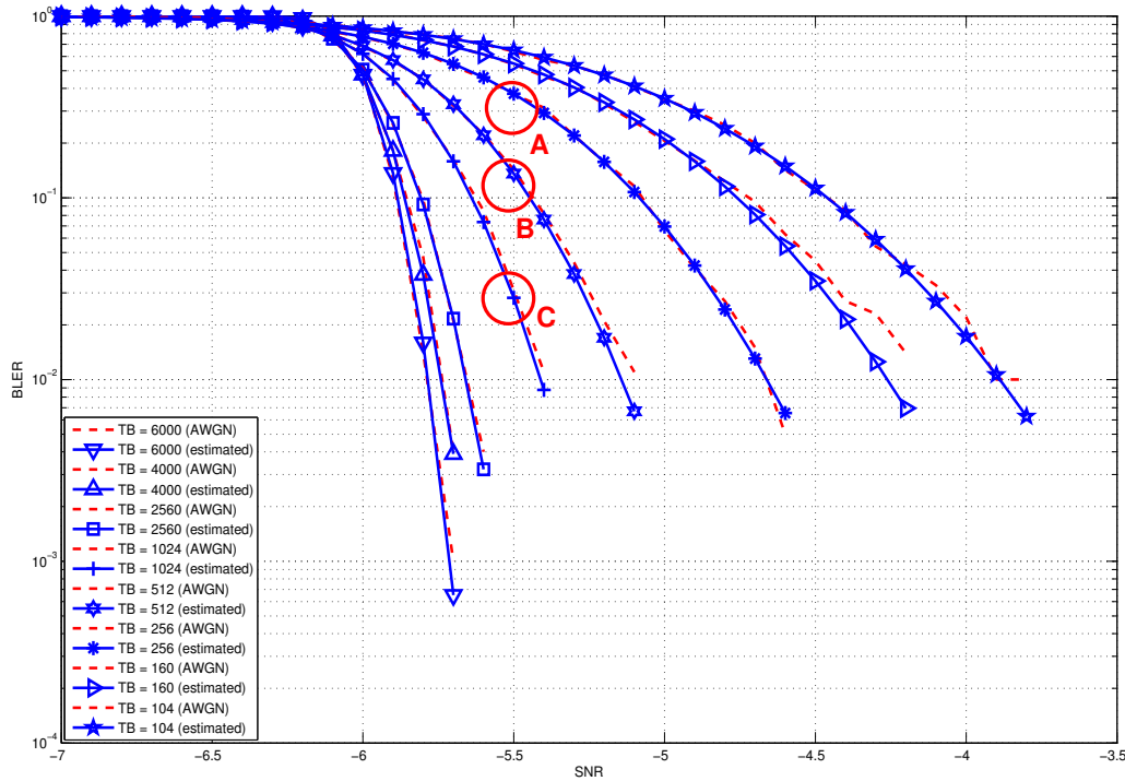
Figure 17.51: BLER for tests 1, 2, 3.
