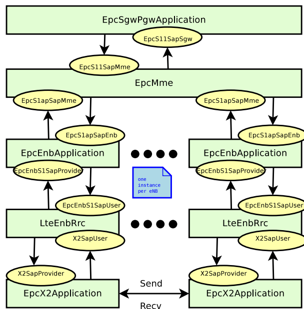
Figure 17.9: EPC control model
