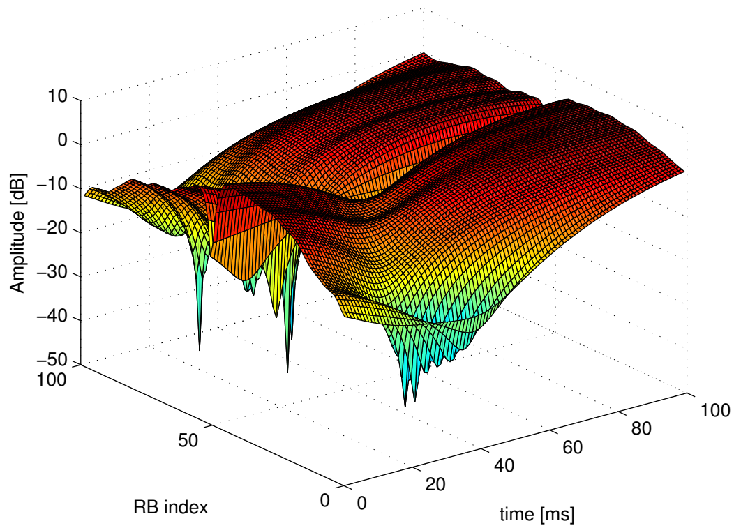
Figure 17.43: Excerpt of the fading trace included in the simulator for a pedestrian scenario (speed of 3 kmph).
