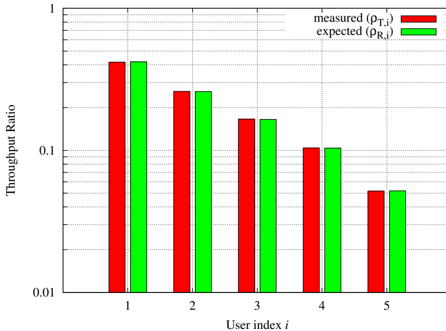
Figure 17.50: Throughput ratio evaluation for the PF scheduler in a scenario where the UEs have MCS index 28, 24, 16, 12, 6
