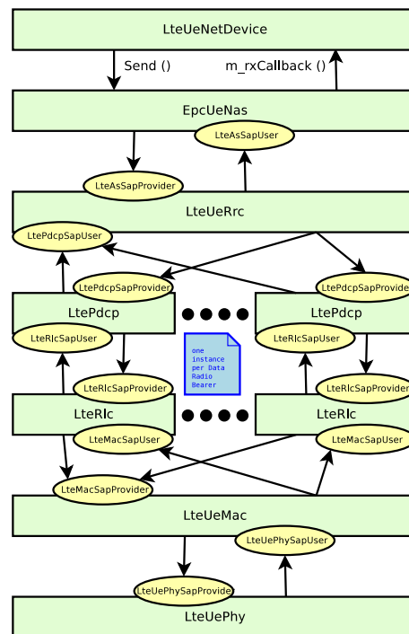
Figure 17.2: LTE radio protocol stack architecture for the UE on the data plane
