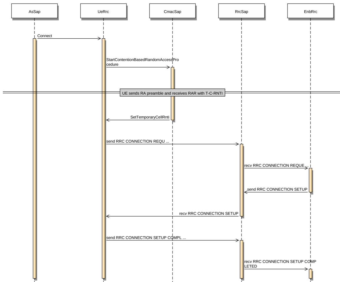
Figure 17.33: Sequence diagram of the RRC Connection Establishment procedure
