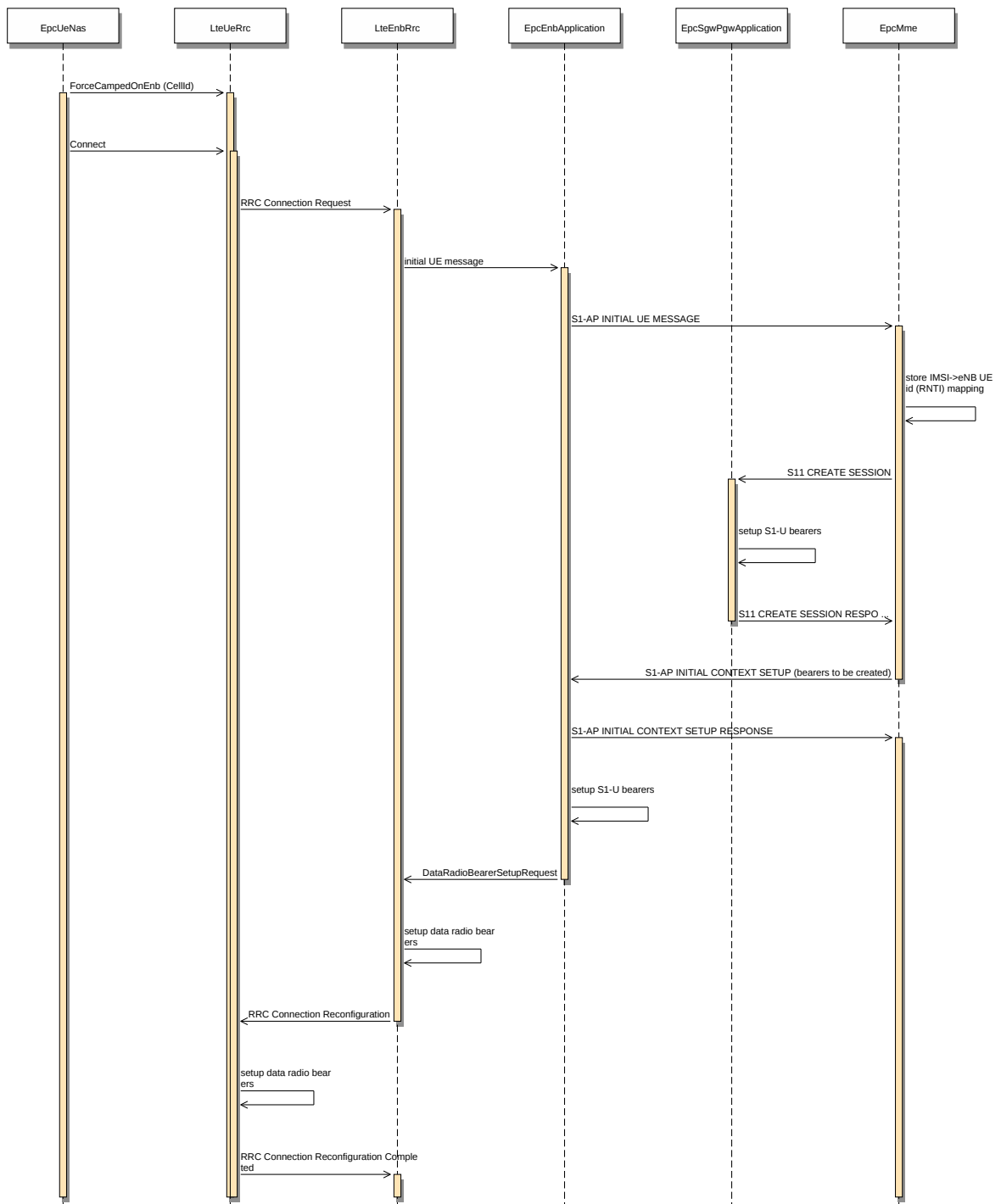
Figure 17.36: Sequence diagram of the attach procedure
