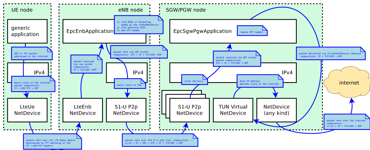
Figure 17.38: Data flow in the uplink between the UE and the internet
