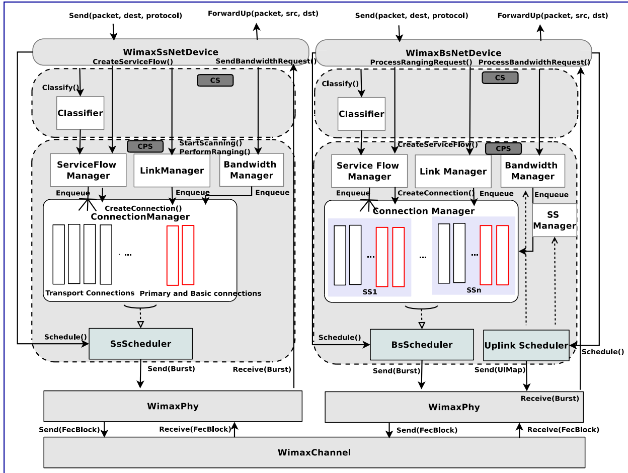
Figure 30.1: WiMAX architecture
