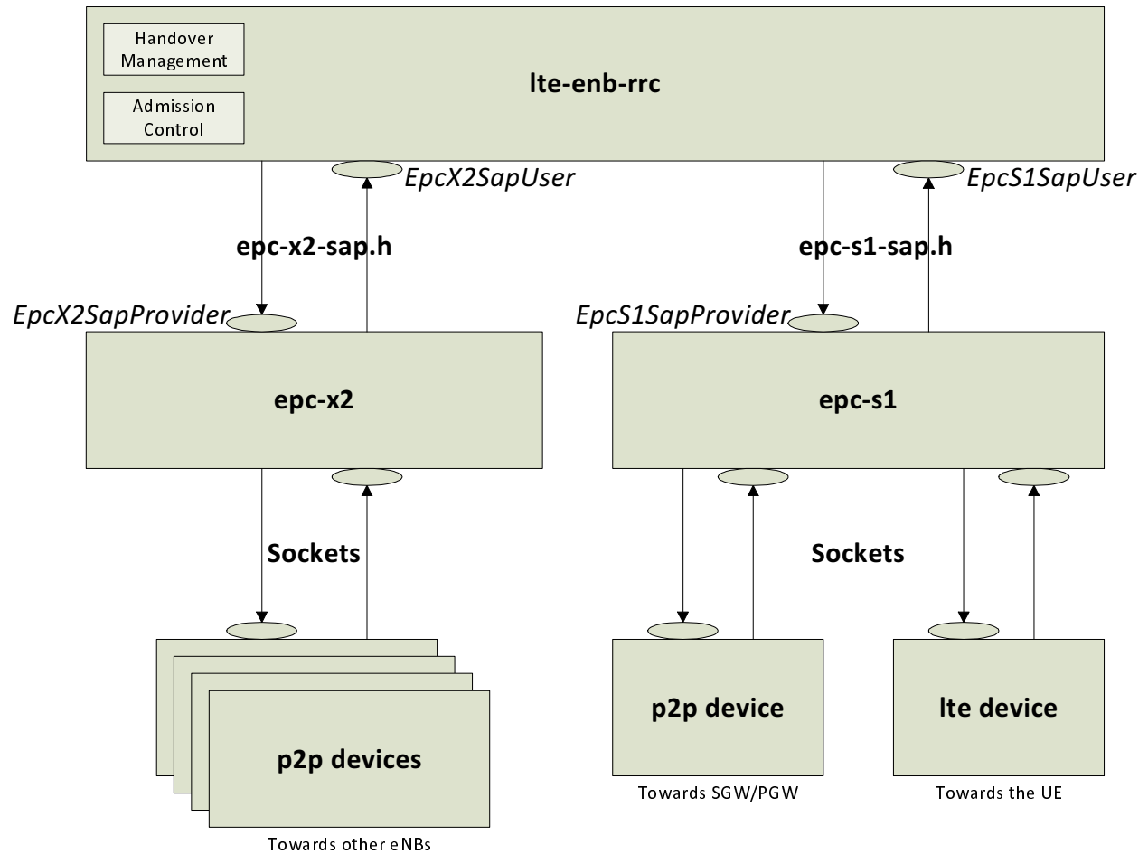
Figure 17.40: Implementation Model of X2 entity and SAPs
