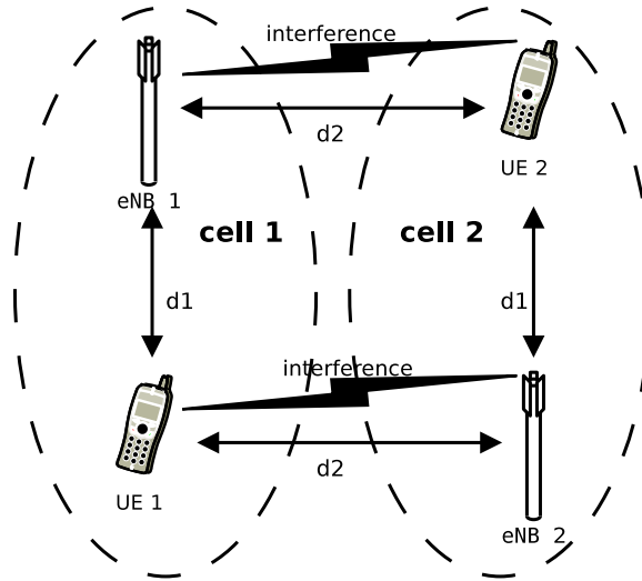
Figure 17.48: Topology for the inter-cell interference test
