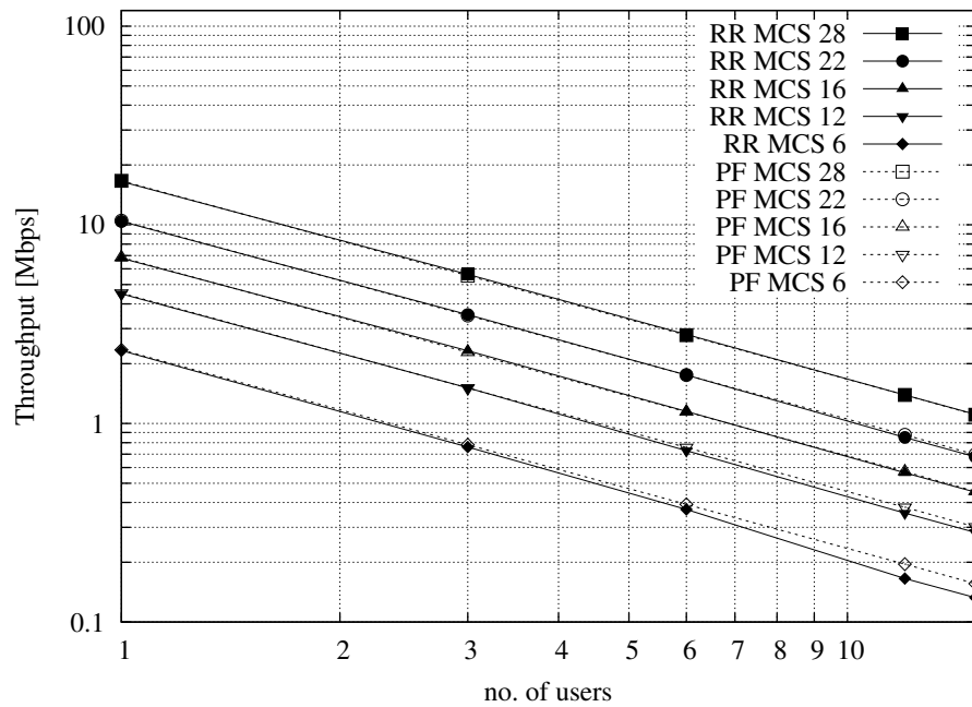
Figure 17.49: Test vectors for the RR and PF Scheduler in the downlink in a scenario where all UEs use the same MCS.
