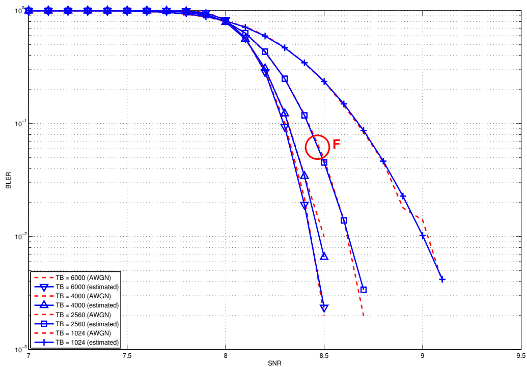
Figure 17.53: BLER for test 6.
