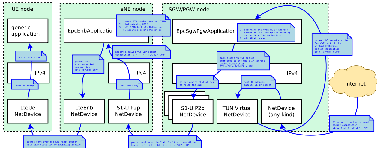
Figure 17.37: Data flow in the downlink between the internet and the UE
