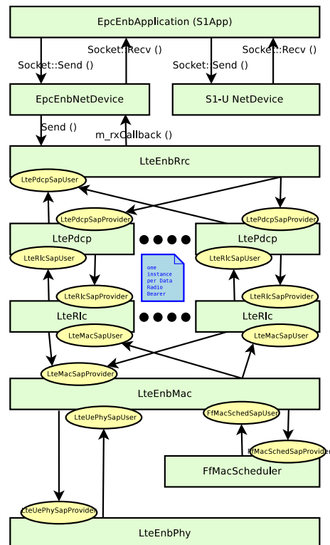
Figure 17.5: LTE radio protocol stack architecture for the eNB on the data plane
