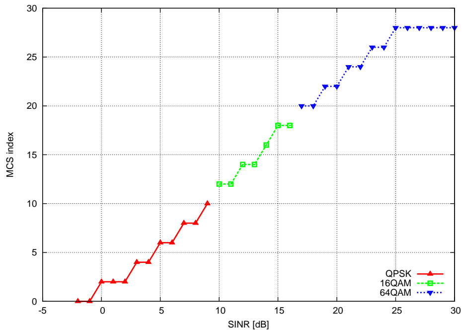
Figure 17.47: Test vector for Adaptive Modulation and Coding
