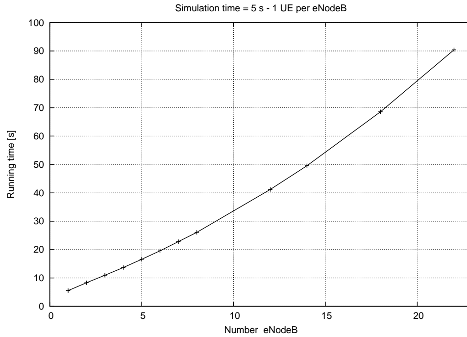
Figure 17.60: Running time
