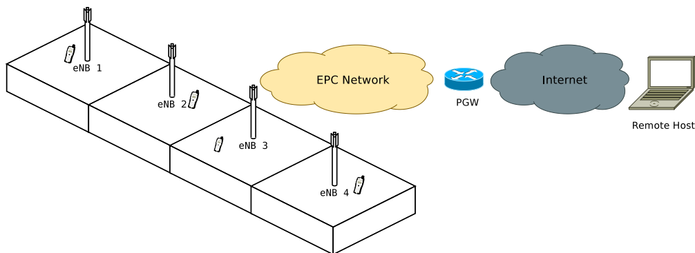
Figure 17.55: Propagation Model
