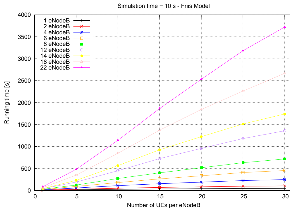
Figure 17.56: Running time
