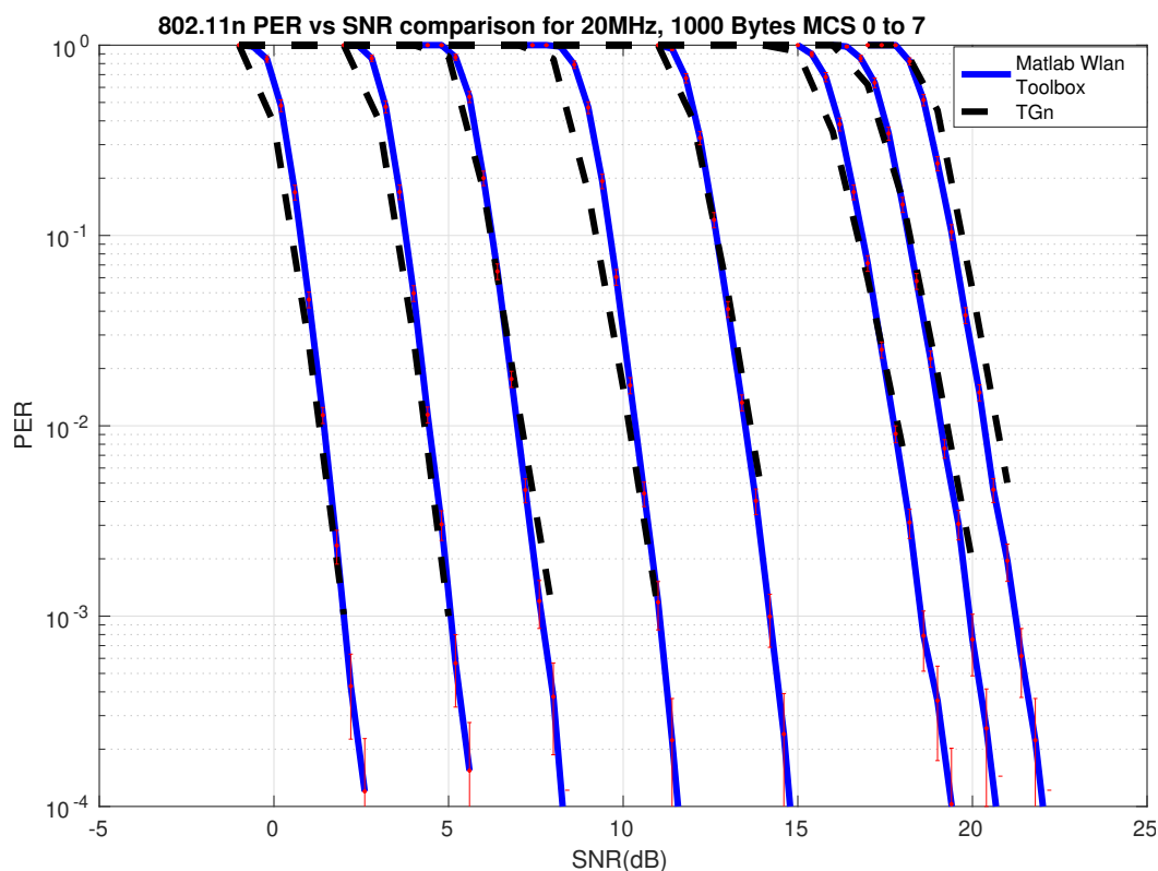
Fig. 3: Comparison of table-based OFDM Error Model with TGn results.
