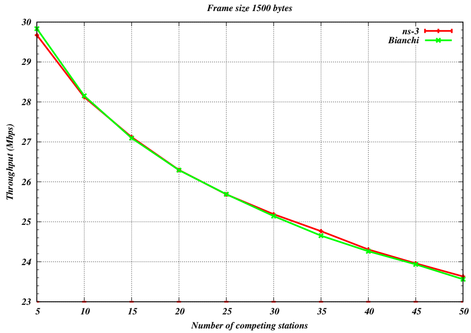
Fig. 10: Bianchi throughput validation results for 802.11a 54 Mbps in adhoc configuration
