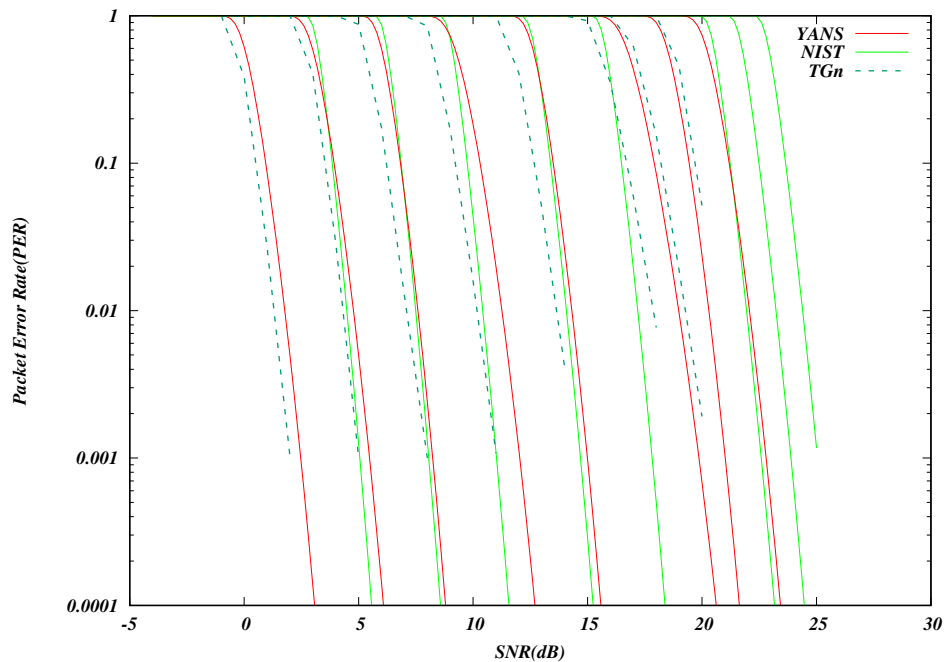
Fig. 4: YANS and NIST error model comparison with TGn results
