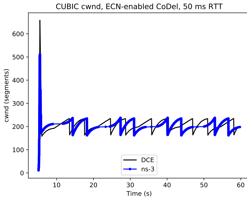
Fig. 13: CUBIC cwnd evolution for 50ms/50Mbps bottleneck, with ECN
