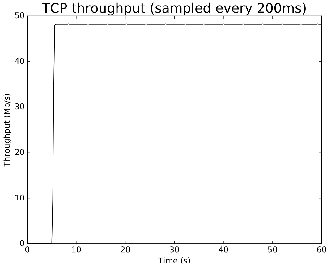
Fig. 10: DCTCP throughput for 10ms/50Mbps bottleneck, 1ms CE threshold
