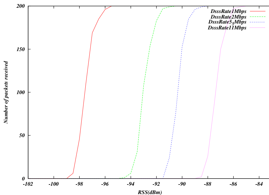
Fig. 5: Clear channel (AWGN) error model for 802.11b
