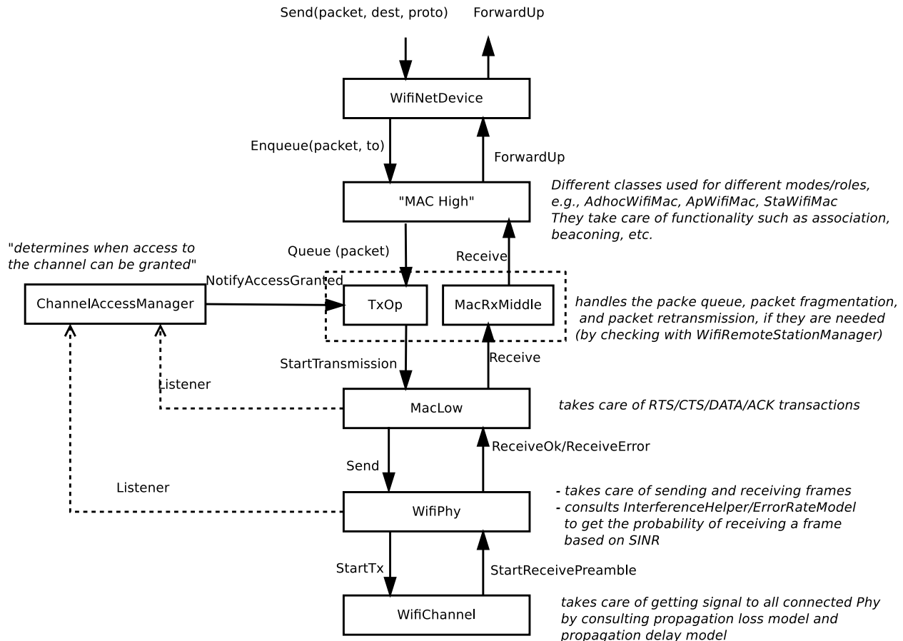
Fig. 1: WifiNetDevice architecture.
