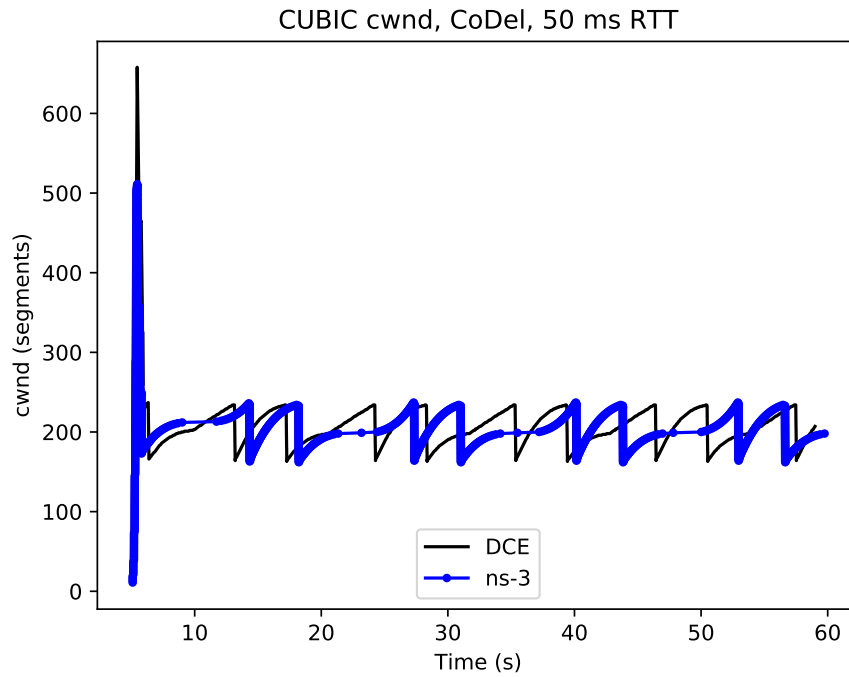
Fig. 12: CUBIC cwnd evolution for 50ms/50Mbps bottleneck, no ECN
