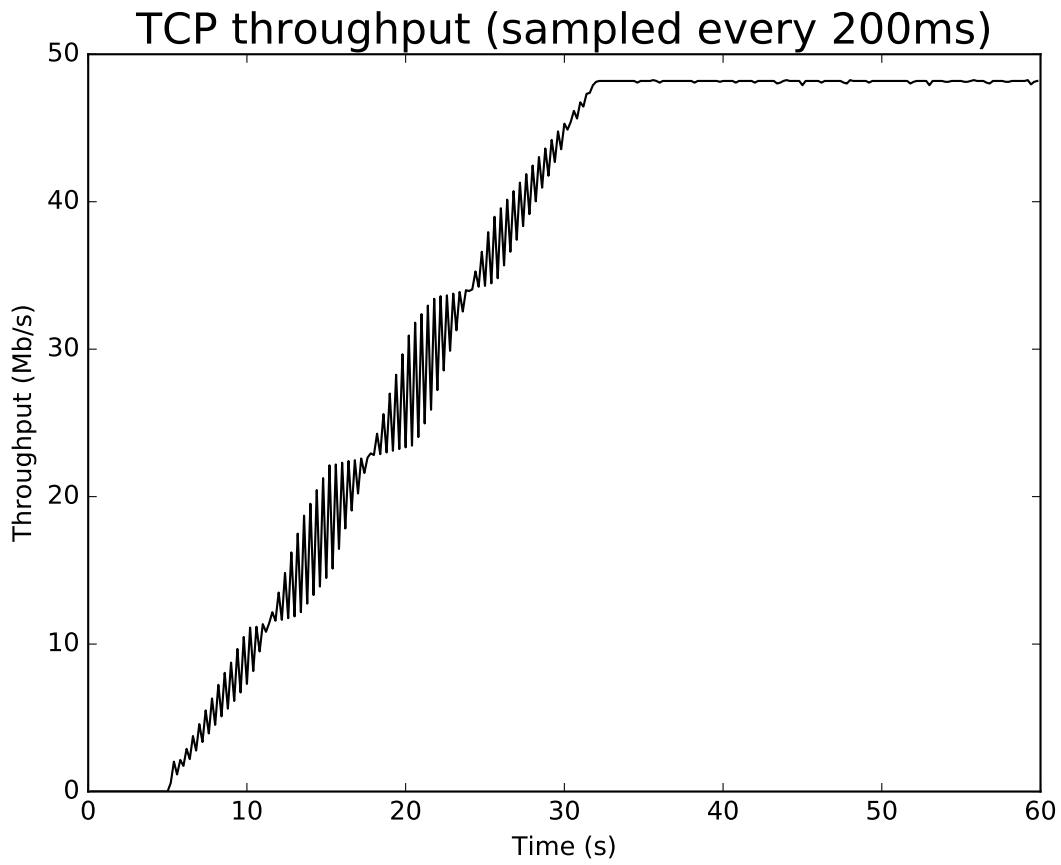
Fig. 11: DCTCP throughput for 80ms/50Mbps bottleneck, 1ms CE threshold
