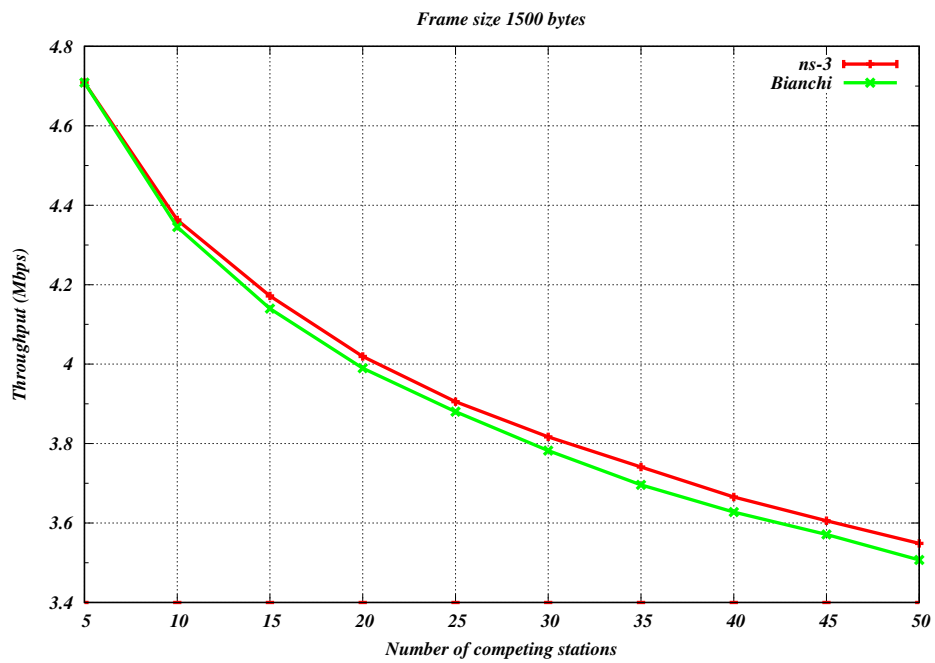
Fig. 11: Bianchi throughput validation results for 802.11g 6 Mbps in infrastructure configuration
