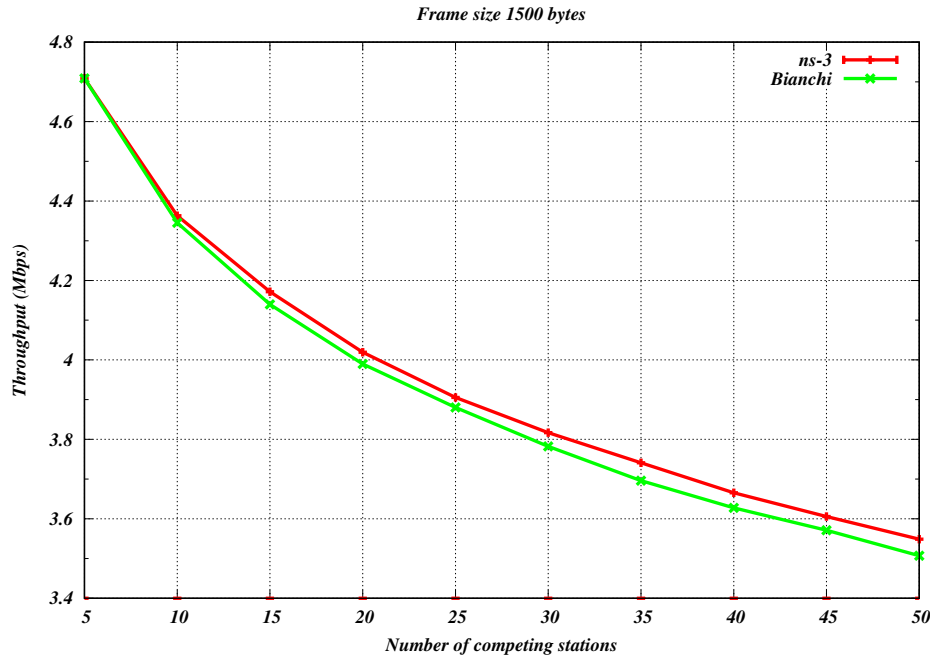
Fig. 18: Bianchi throughput validation results for 802.11g 6 Mbps in infrastructure configuration
