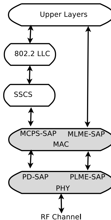
Fig. 1: Architecture and scope of lr-wpan models
