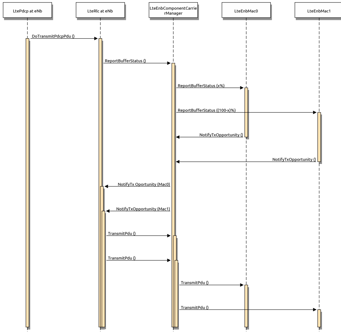
Fig. 64: Sequence Diagram of downlink buffer status reporting (BSR) with CA
