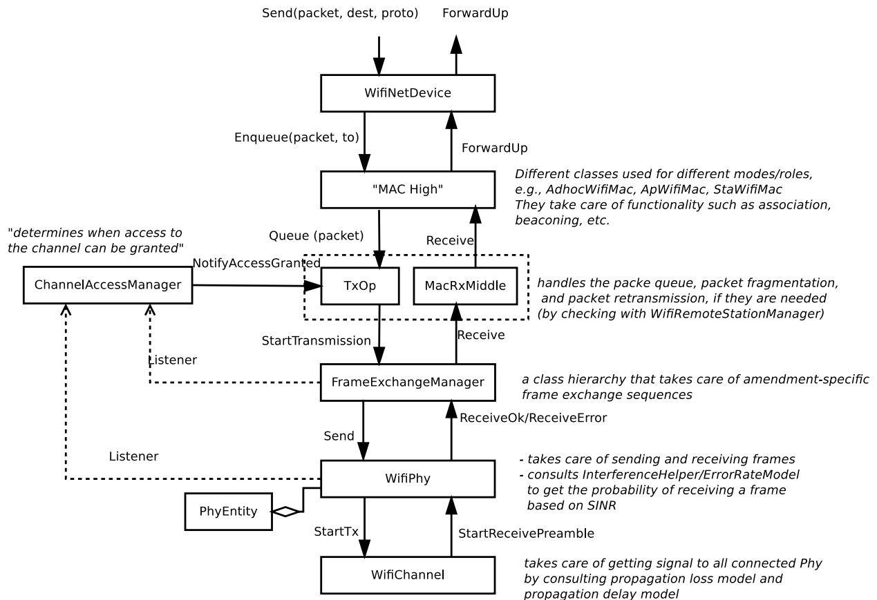
Fig. 1: WifiNetDevice architecture
