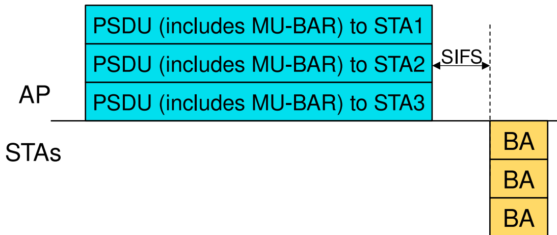
Fig. 10: Acknowledgment of DL MU frames via aggregated MU-BAR Trigger Frames
