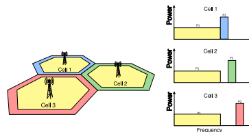
Fig. 52: Strict Frequency Reuse scheme
