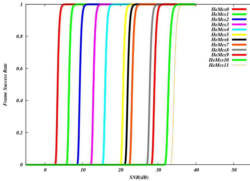
Fig. 16: Frame error rate (NIST model) for 802.11ax (HE OFDM) Wi-Fi
