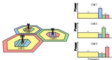
Fig. 55: Soft Fractional Fractional Frequency Reuse scheme
