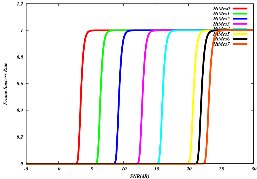
Fig. 14: Frame error rate (NIST model) for 802.11n (HT OFDM) Wi-Fi
