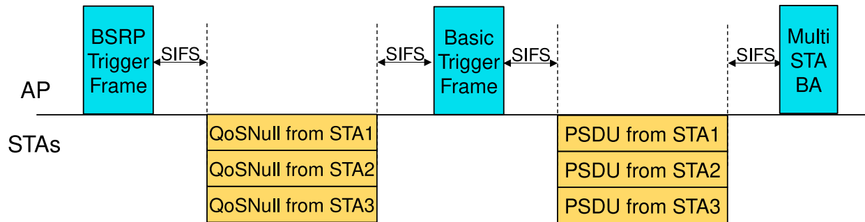
Fig. 11: Acknowledgment of DL MU frames via aggregated MU-BAR Trigger Frames
