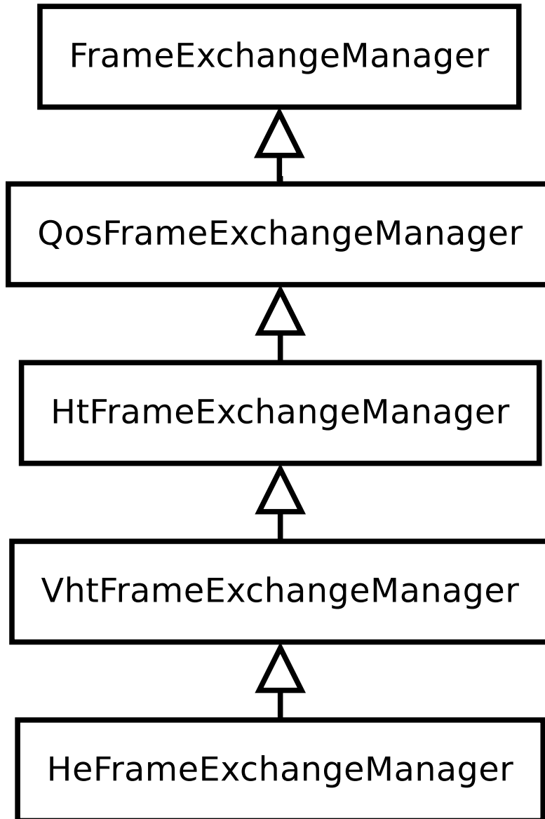
Fig. 7: FrameExchangeManager hierarchy
