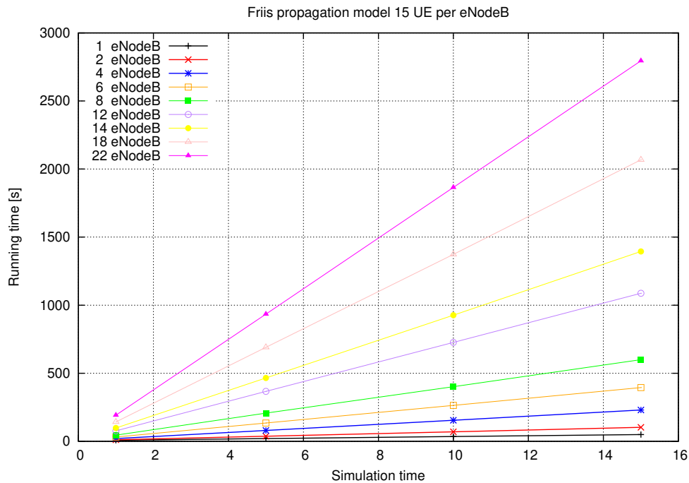
Fig. 105: Simulation time
