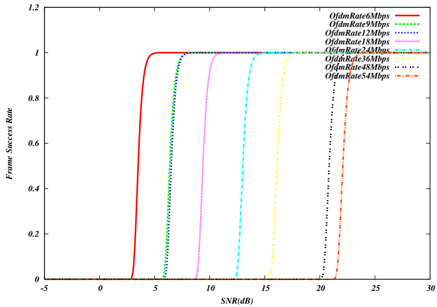
Fig. 13: Frame error rate (NIST model) for 802.11a/g (OFDM) Wi-Fi
