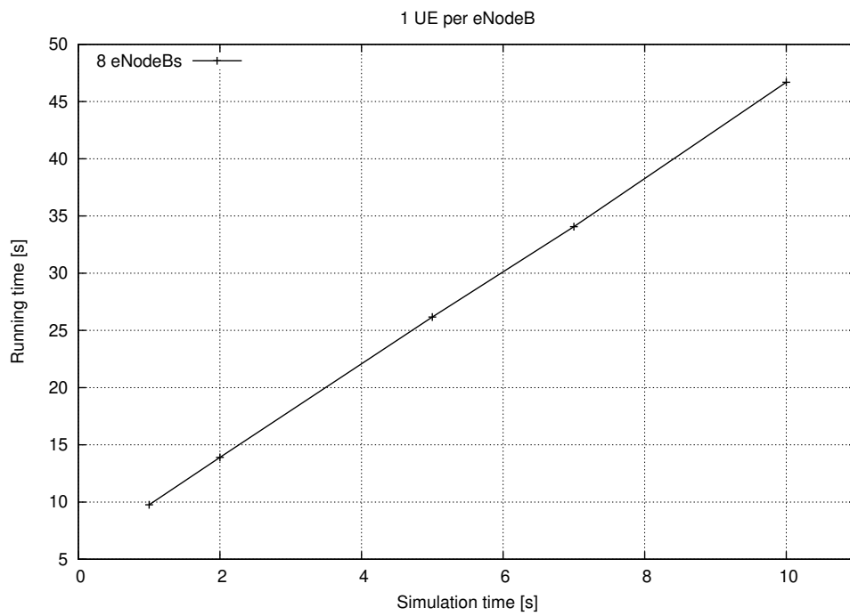
Fig. 109: Simulation time
