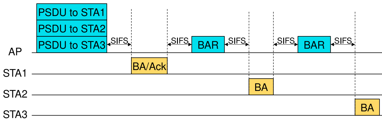
Fig. 8: Acknowledgment of DL MU frames in single-user format
