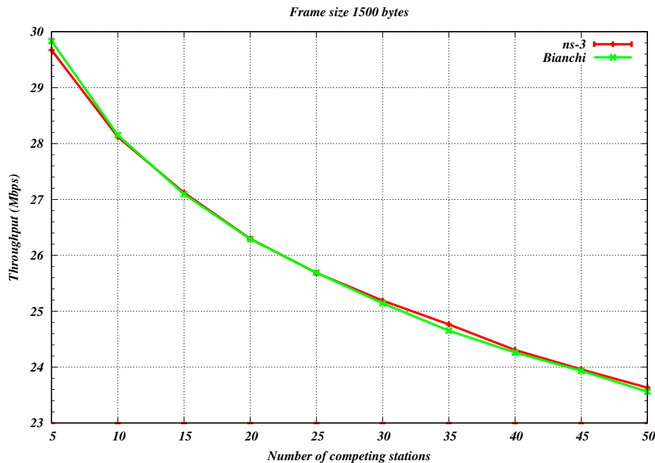
Fig. 17: Bianchi throughput validation results for 802.11a 54 Mbps in adhoc configuration
