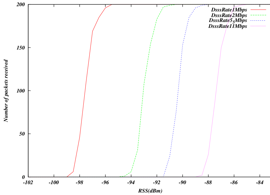
Fig. 12: Clear channel (AWGN) error model for 802.11b
