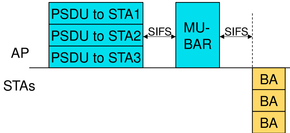
Fig. 9: Acknowledgment of DL MU frames via MU-BAR Trigger Frame sent as single-user frame
