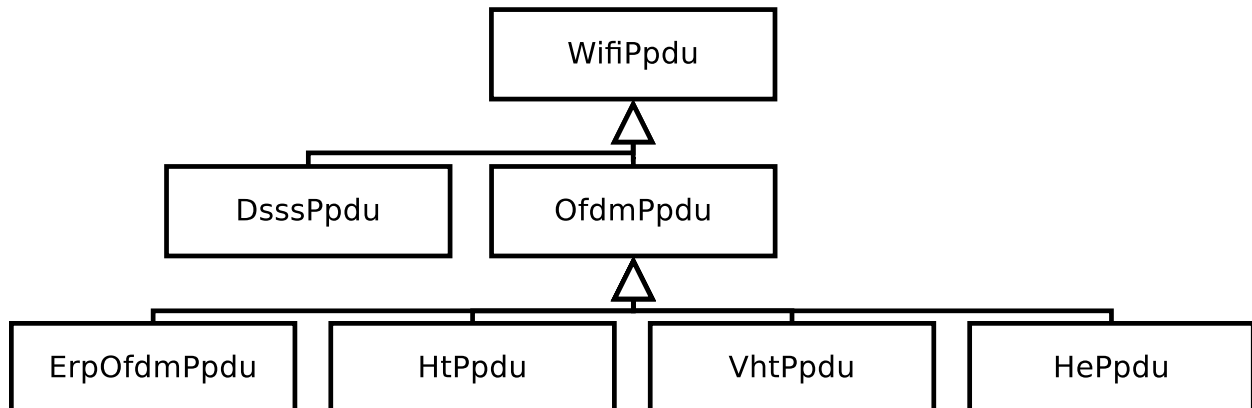
Fig. 3: WifiPpdu hierarchy
