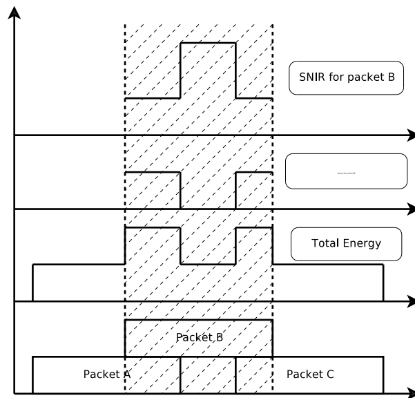
Figure 12.2: SNIR function over time
