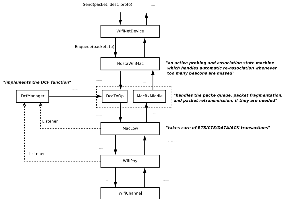
Figure 12.1: Wifi NetDevice architecture.
