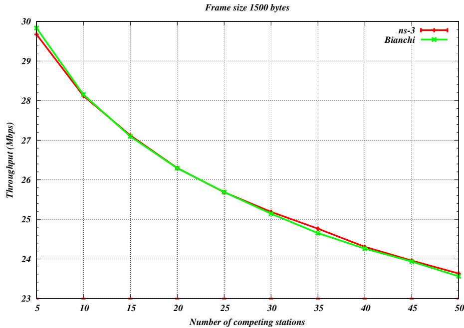
Fig. 23: Bianchi throughput validation results for 802.11a 54 Mbps in adhoc configuration
