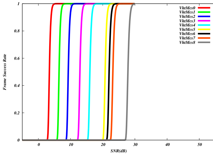
Fig. 21: Frame error rate (NIST model) for 802.11ac (VHT OFDM) Wi-Fi
