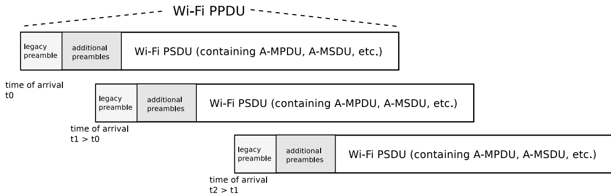
Fig. 17: WifiPhyRxTraceHelper scenario of interest
