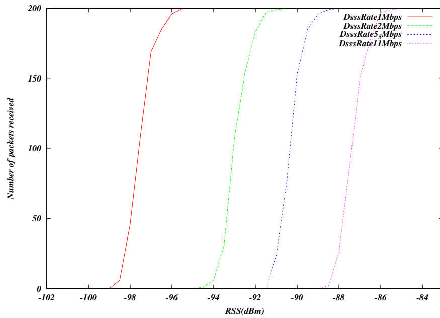
Fig. 18: Clear channel (AWGN) error model for 802.11b
