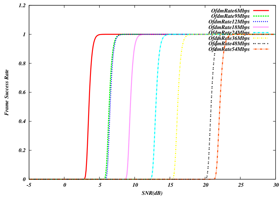
Fig. 19: Frame error rate (NIST model) for 802.11a/g (OFDM) Wi-Fi
