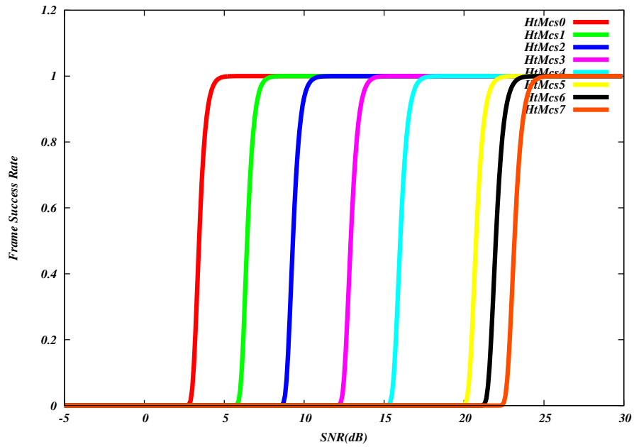
Fig. 20: Frame error rate (NIST model) for 802.11n (HT OFDM) Wi-Fi
