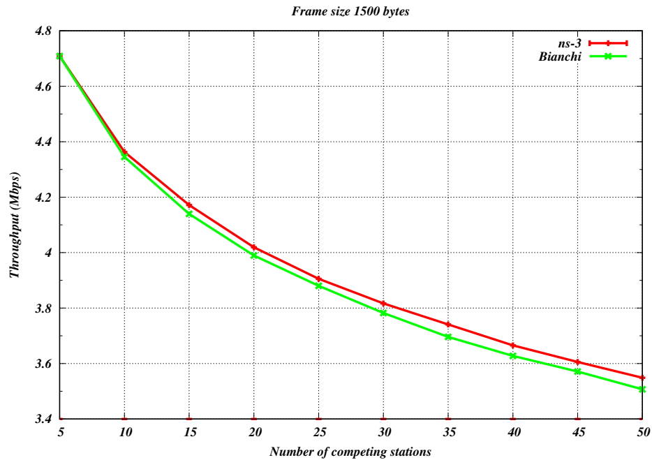
Fig. 24: Bianchi throughput validation results for 802.11g 6 Mbps in infrastructure configuration
