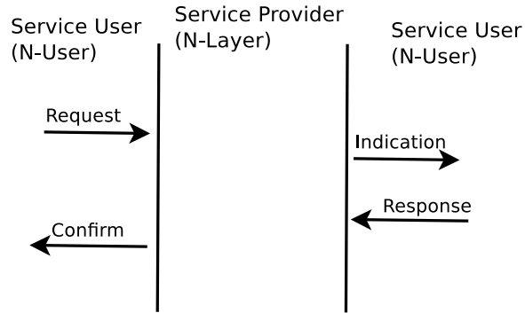
Fig. 2: Service primitives
