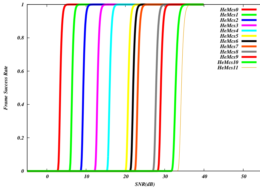
Fig. 22: Frame error rate (NIST model) for 802.11ax (HE OFDM) Wi-Fi
