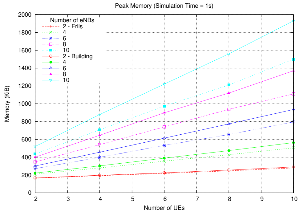
Fig. 106: Memory profile
