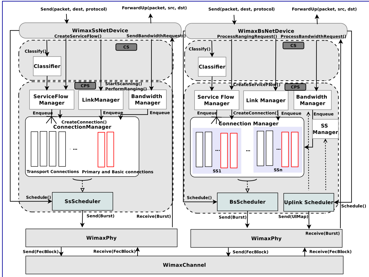
Fig. 1: WiMAX architecture
