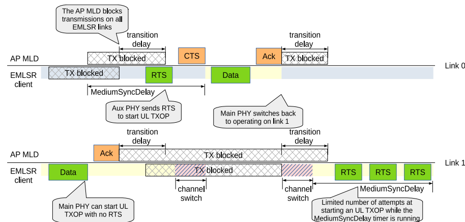
Fig. 16: EMLSR operations: Uplink TXOP
