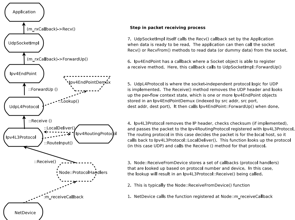
Figure 9.3: Receive path of a packet.
