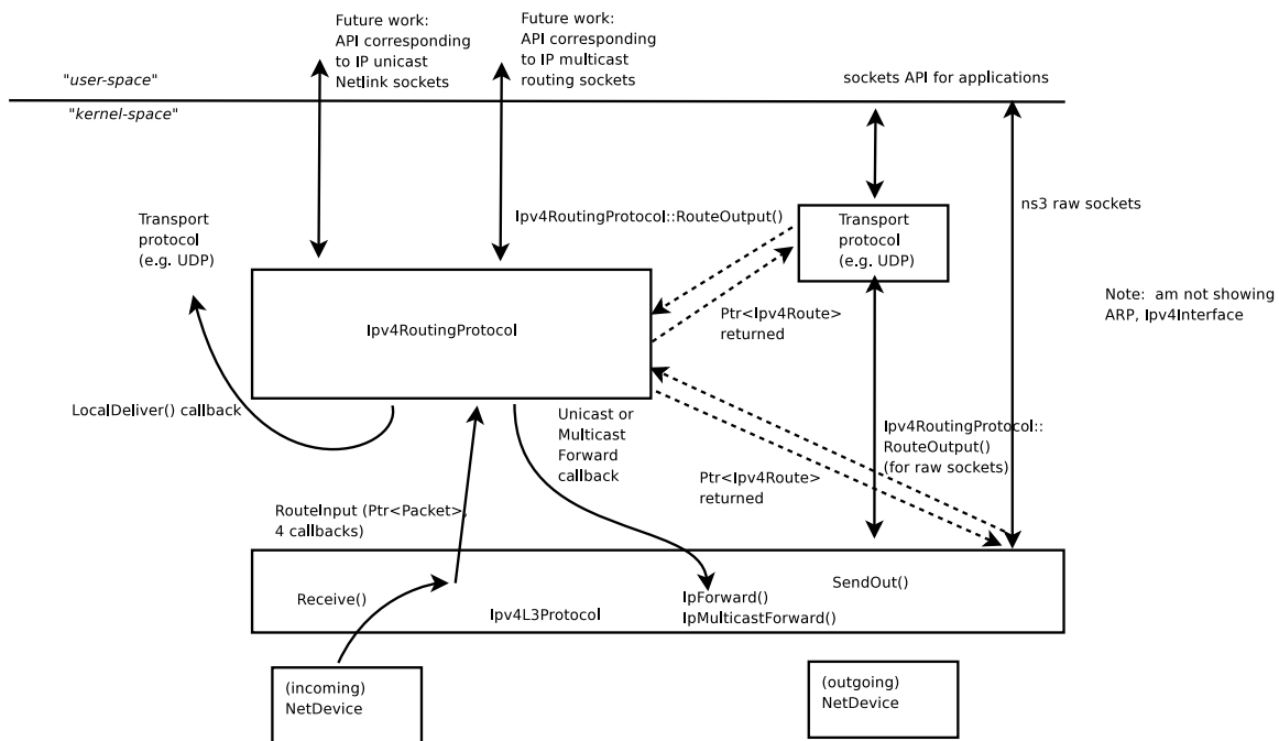
Figure 11.1: Overview of routing
