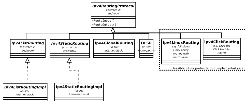
Figure 11.2: Ipv4Routing specialization
