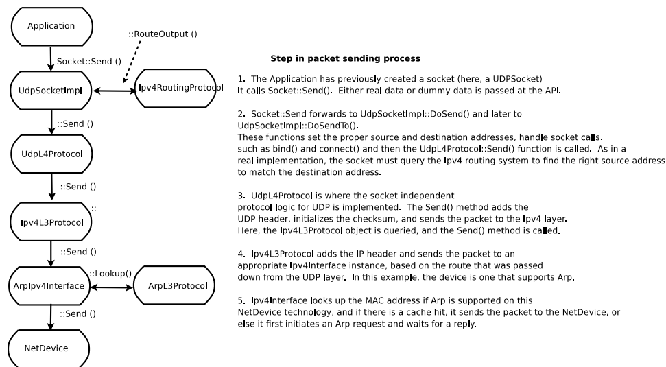
Figure 9.2: Send path of a packet.
