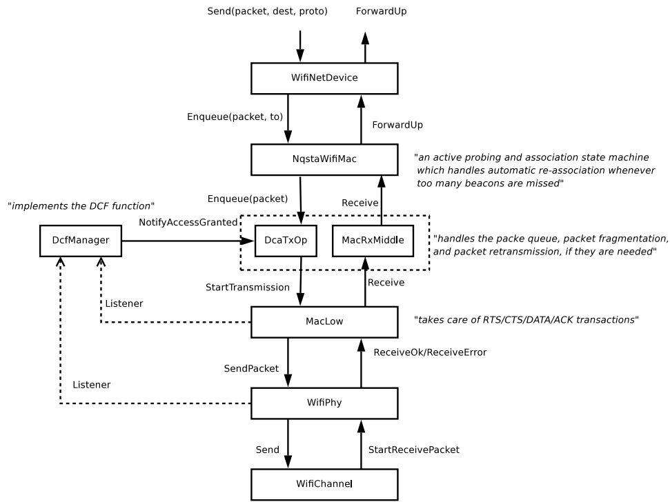
Figure 12.1: Wifi NetDevice architecture.
