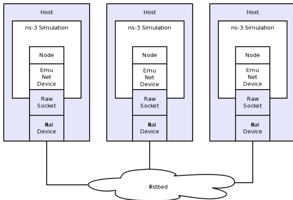
Figure 21.1: Example Implementation of Testbed Emulation.
