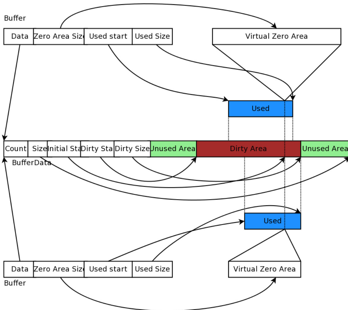
Figure 11.2: Implementation overview of a packet's byte Buffer.
