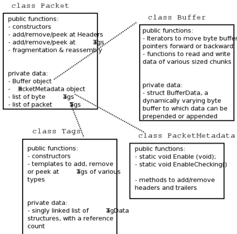
Figure 11.1: Implementation overview of Packet class.
