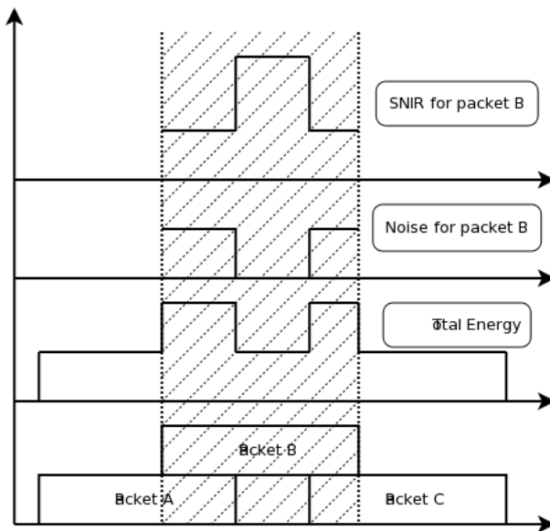
Figure 18.2: SNIR function over time
