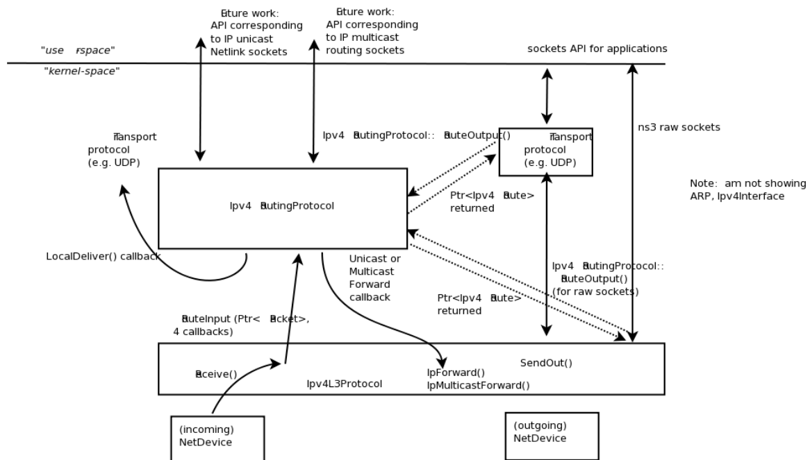
Figure 28.1: Overview of routing
