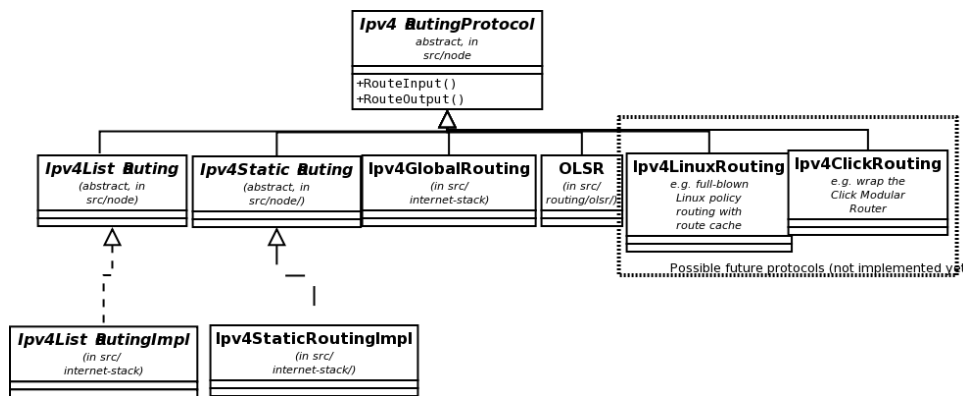
Figure 28.2: Ipv4Routing specialization
