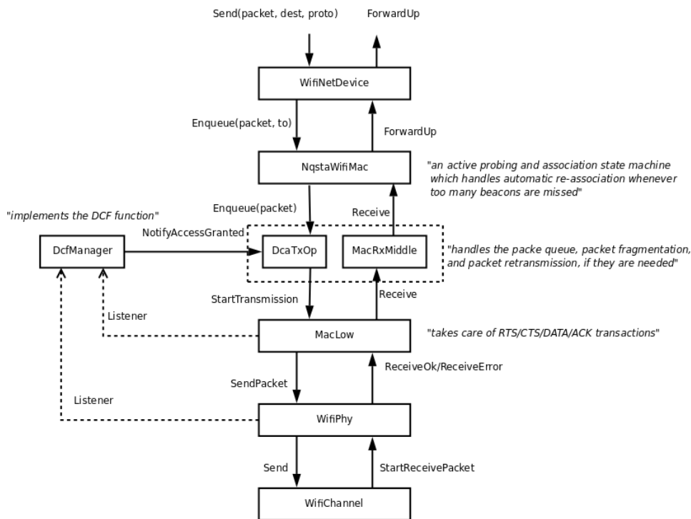
Figure 18.1: Wifi NetDevice architecture.
