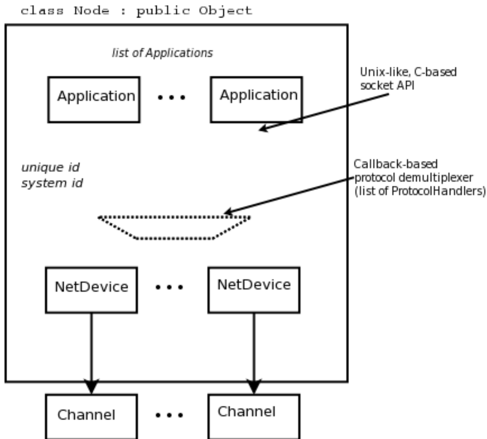
Figure 14.1: High-level node architecture.
