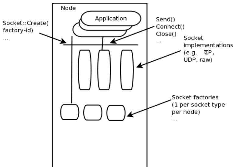
Figure 24.1: Implementation overview of native sockets API
