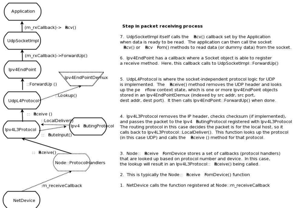
Figure 25.2: Receive path of a packet.
