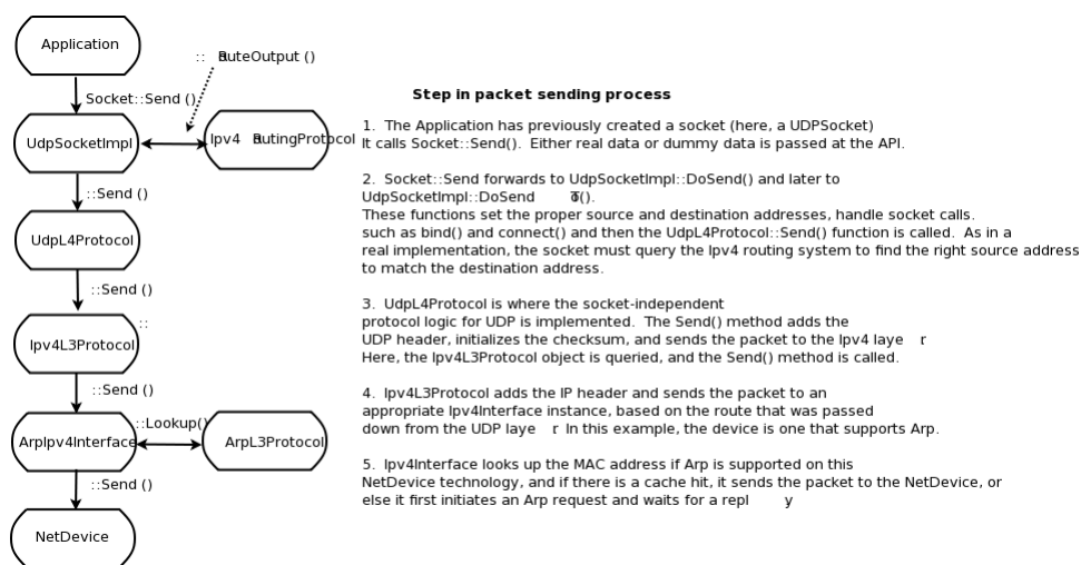
Figure 25.1: Send path of a packet.
