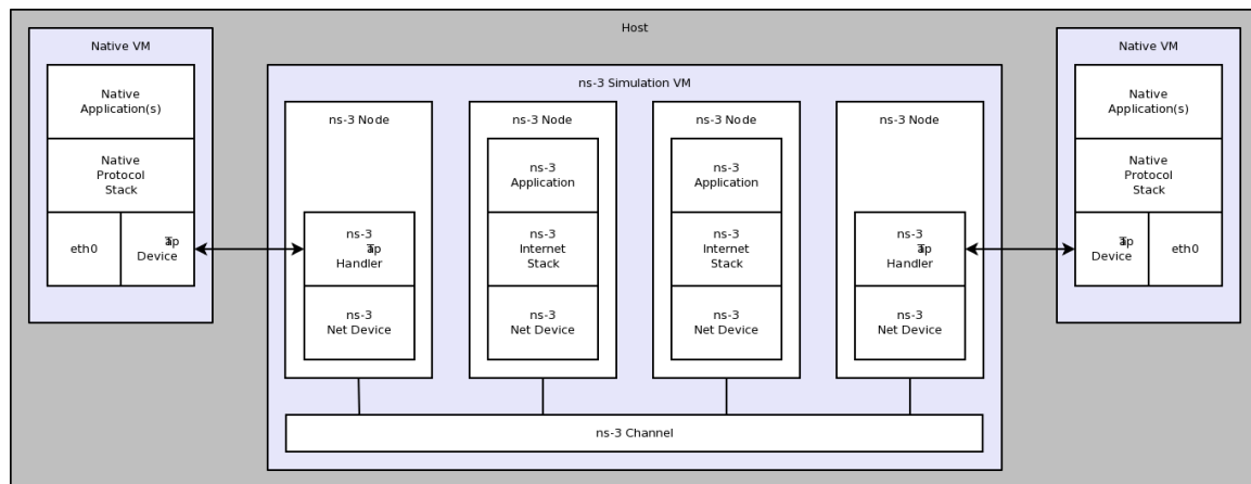
Figure 21.2: Implementation overview of emulated channel.
